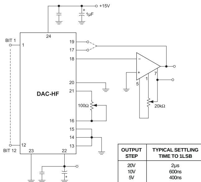
Figure 7. Unipolar Fast Voltage Output Circuit
