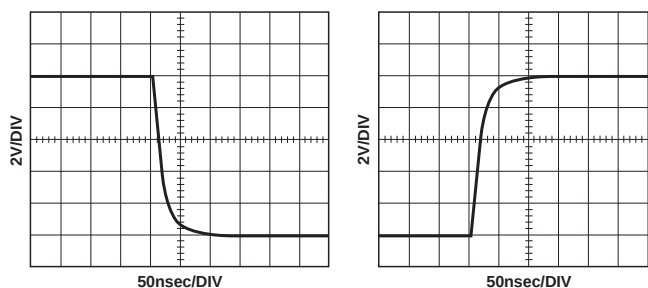
DAC-HF with AM-500, \pm 5V output full scale (10V) step
