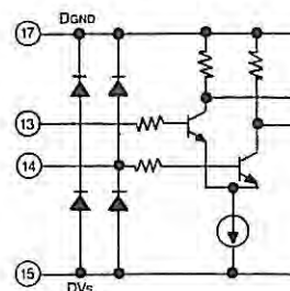
Figure 1. Clock Inputs
