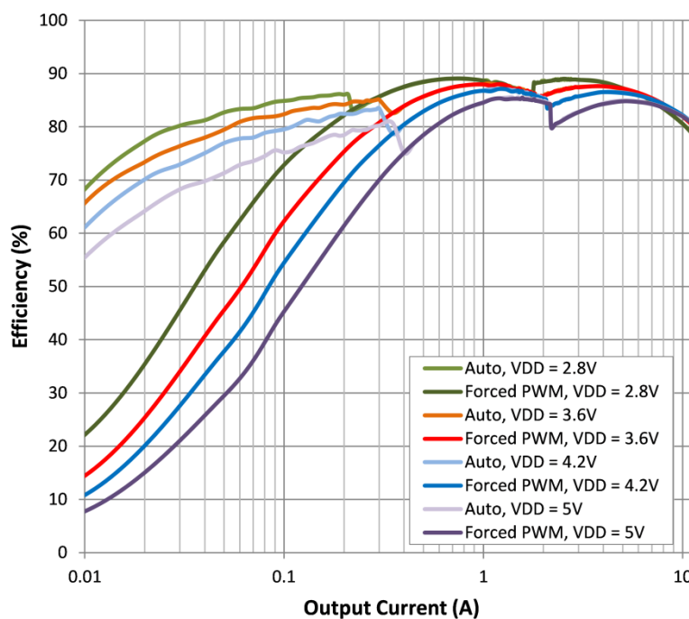
Figure 7: Efficiency vs Output Current V_{OUT} = 0.9\text{ V}
