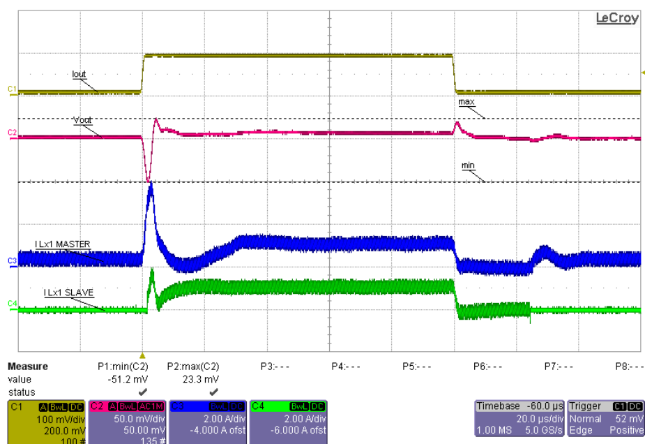
Figure 27: Transient Load, Auto, 4-phases 1 to 5 A in 10 A/μs, V_{DD} = 3.7 V, V_{OUT} = 1.0 V
