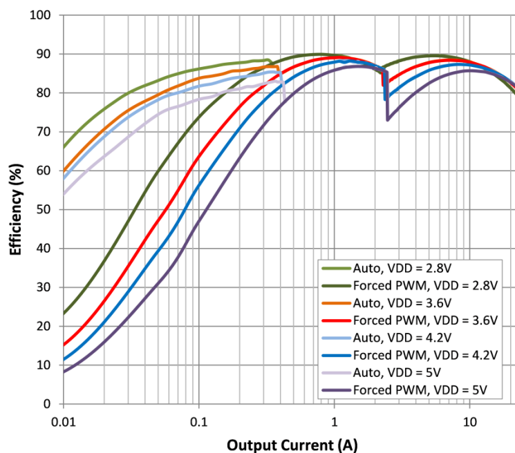
Figure 8: Efficiency vs Output Current V_{OUT} = 1.0\text{ V} , dual parallel mode (24 A max)
