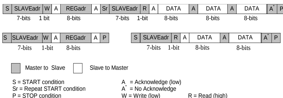
Figure 43: 2-WIRE Page Read
