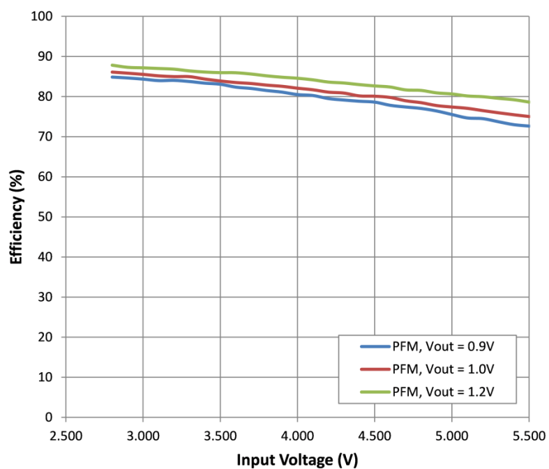
Figure 11: Efficiency vs Input Voltage I_{OUT} = 100\text{ mA}
