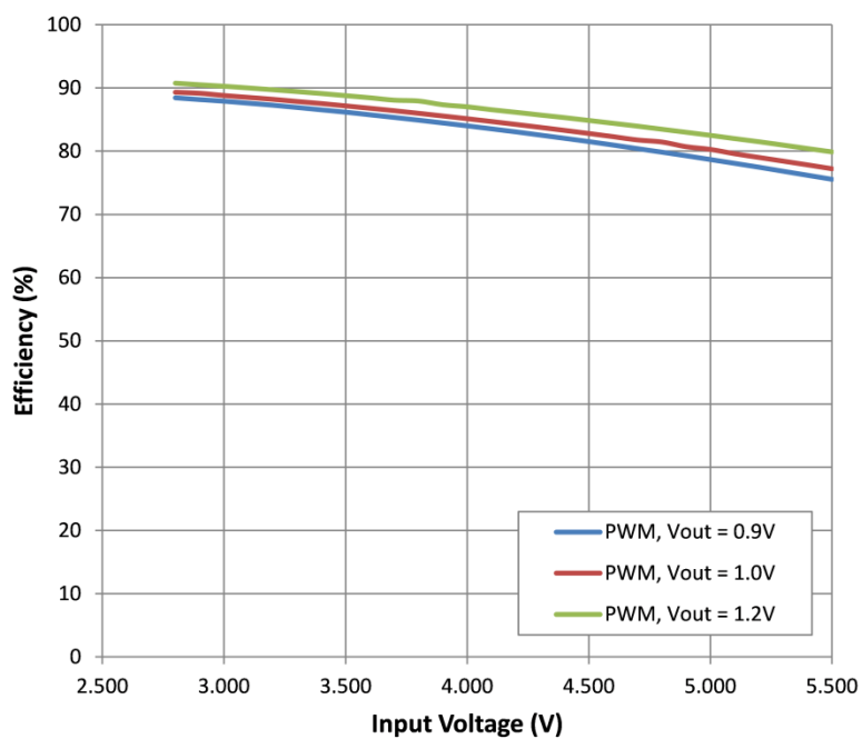
Figure 12: Efficiency vs Input Voltage I_{OUT} = 2\text{ mA}
