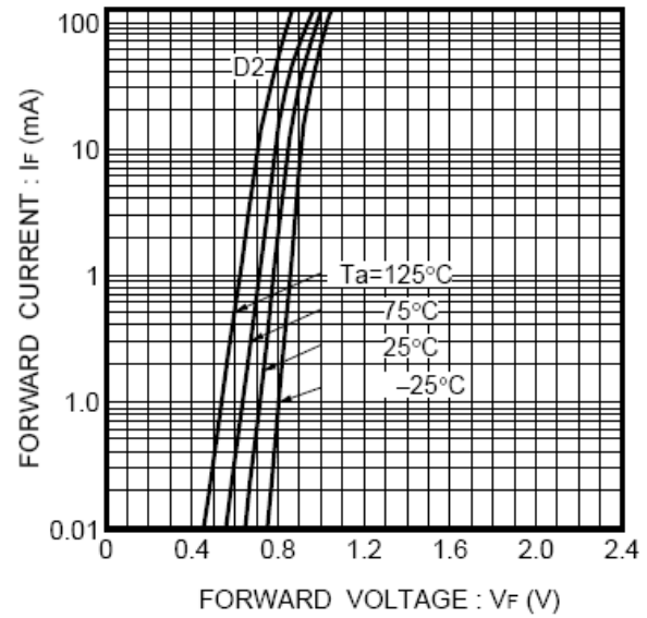
Fig.2 Forward characteristics
