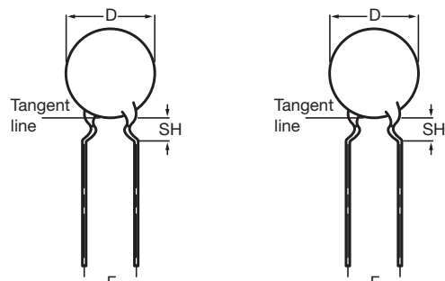
Capacitors with 5 mm (0.20") and 7.5 mm (0.30") lead spacing
