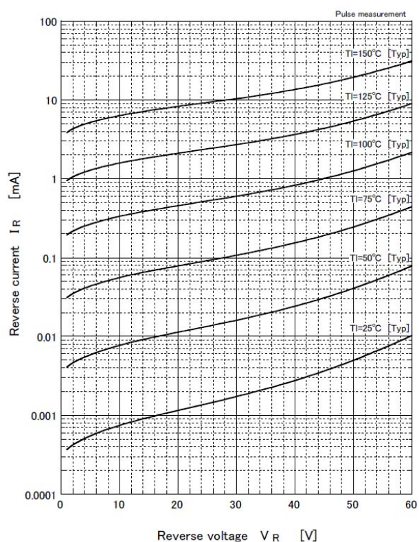
Reverse current
