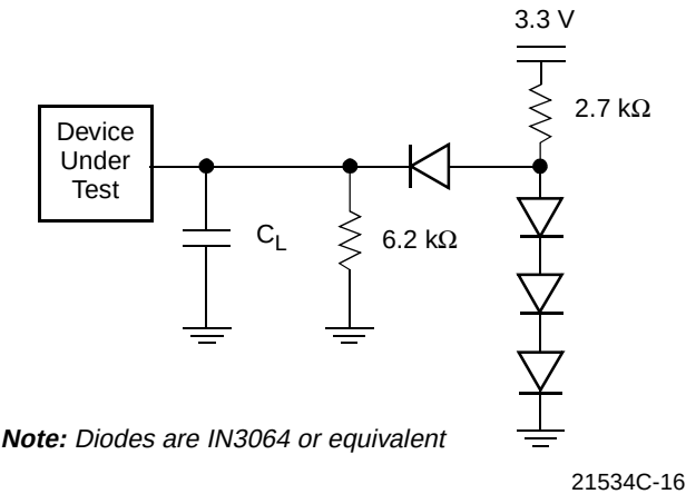
Figure 11. Test Setup
