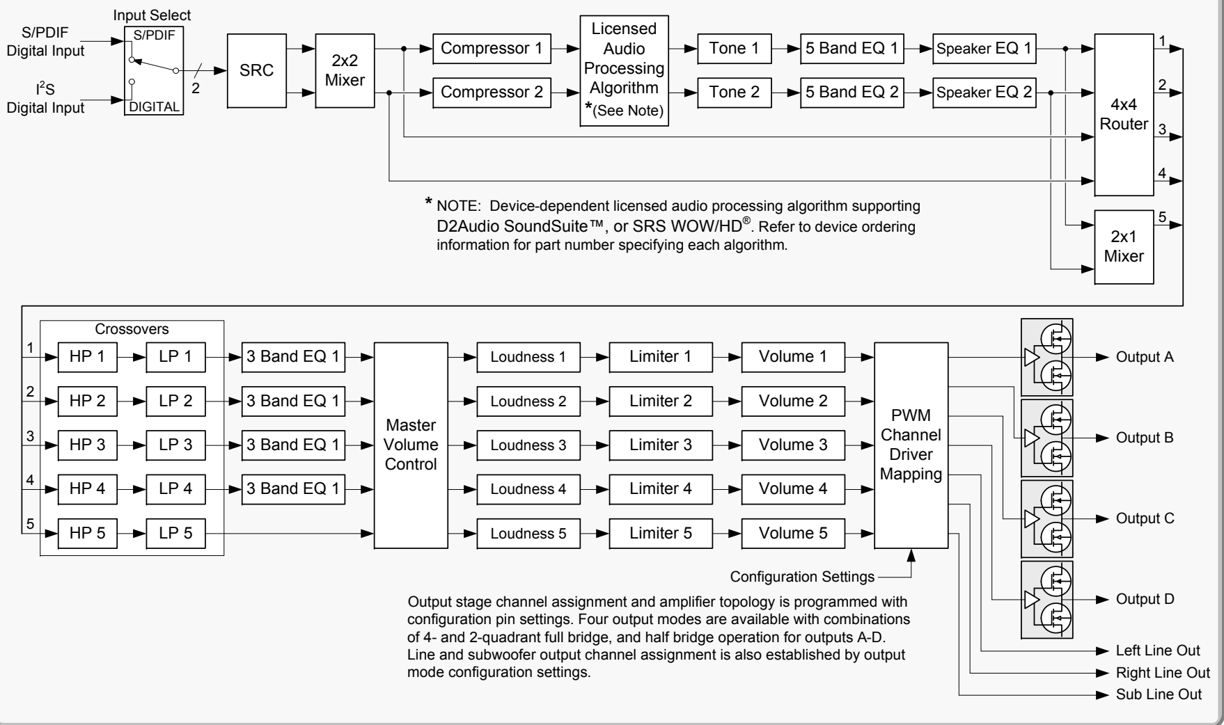
FIGURE 18. D2-45057, D2-45157 AUDIO SIGNAL FLOW
