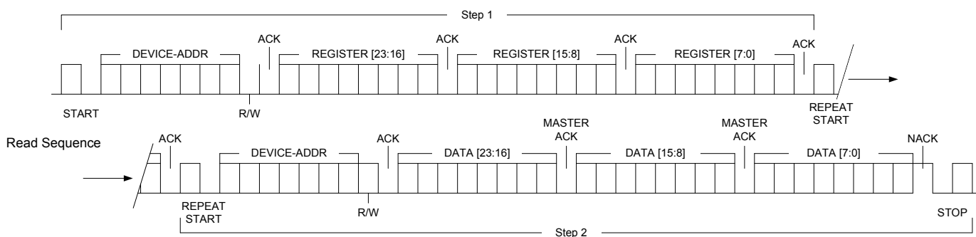
FIGURE 16. I 2 C READ SEQUENCE OPERATION
