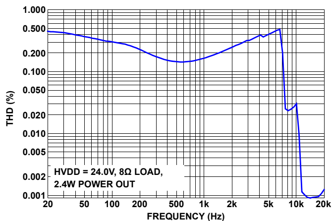
FIGURE 10. THD vs FREQUENCY, HALF-BRIDGE
