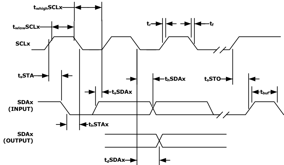
FIGURE 2. I 2 C INTERFACE TIMING
