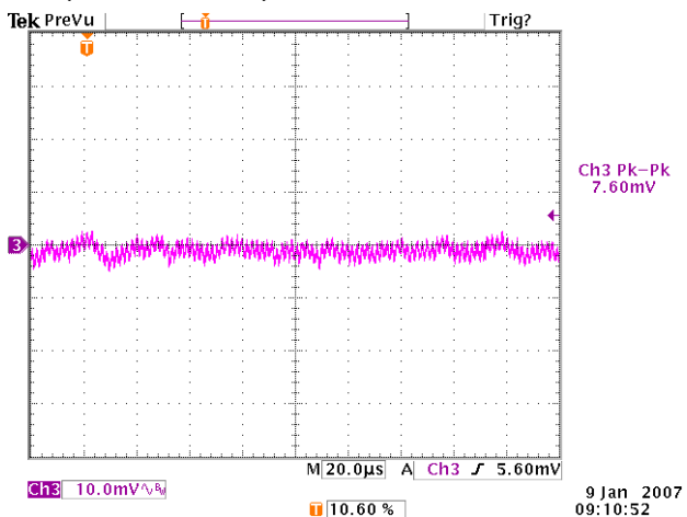
Figure 11: Output ripple & noise at 12Vin, 3.3V/60A out (10mV/div, 1μS/div)
