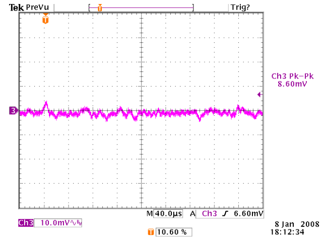
Figure 8: Output ripple & noise at 12Vin, 1.2V/60A out (5mV/div, 1μS/div)
