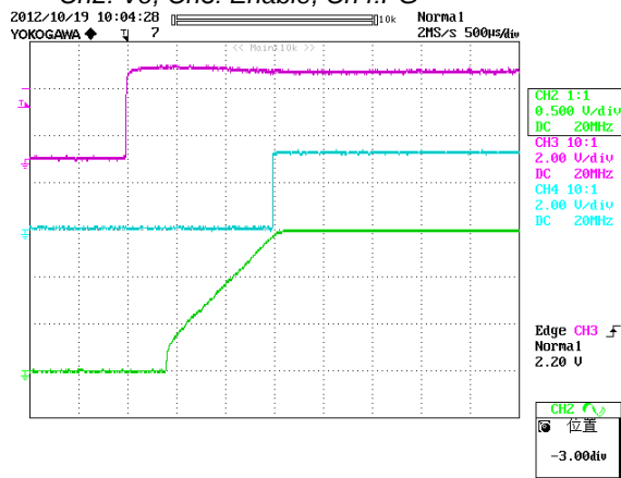
Figure 15: Turn on delay time at 12Vin, 1.5V/60A out (500uS/div) Ch2: Vo, Ch3: Enable, Ch4:PG
