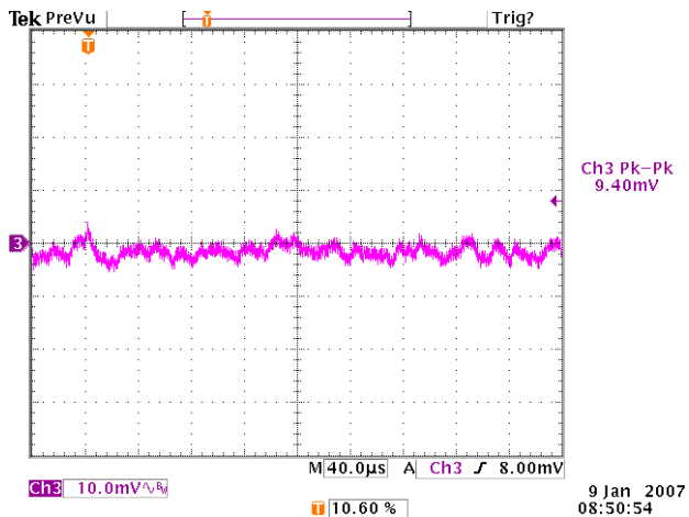
Figure 9: Output ripple & noise at 12Vin, 1.8V/60A out (5mV/div, 1μS/div)
