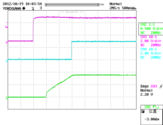
Figure 13: Turn on delay time at 12Vin, 0.9V/60A out (500uS/div) Ch2: Vo, Ch3: Enable, Ch4:PG
