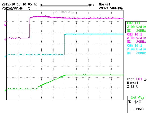
Figure 17: Turn on delay time at 12Vin, 2.5V/60A out (500uS/div) Ch2: Vo, Ch3: Enable, Ch4:PG
