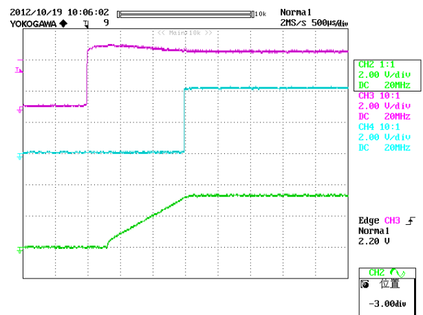
Figure 18: Turn on delay time at 12Vin, 3.3V/60A out (500uS/div) Ch2: Vo, Ch3: Enable, Ch4:PG
