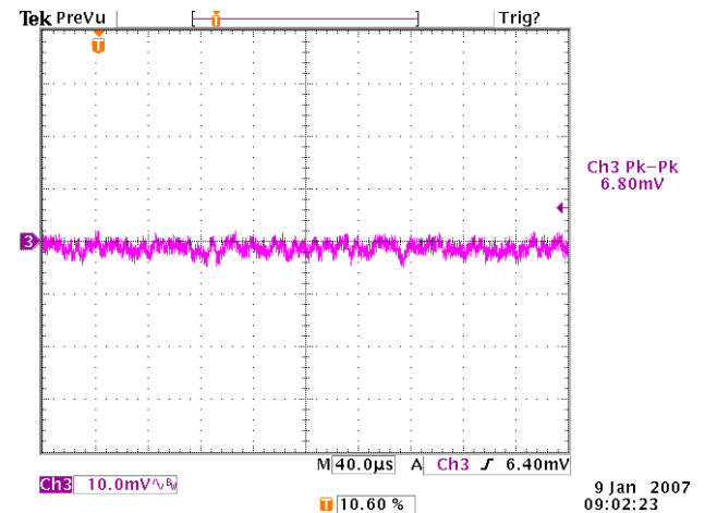
Figure 10: Output ripple & noise at 12Vin, 2.5V/60A out (5mV/div, 1μS/div)
