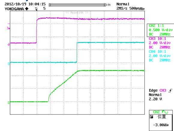
Figure 14: Turn on delay time at 12Vin, 1.2V/60A out (500uS/div) Ch2: Vo, Ch3: Enable, Ch4:PG
