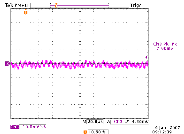
Figure 12: Output ripple & noise at 12Vin, 5.0V/60A out (10mV/div, 1μS/div)
