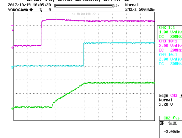
Figure 16: Turn on delay time at 12Vin, 1.8V/60A out (500uS/div) Ch2: Vo, Ch3: Enable, Ch4:PG
