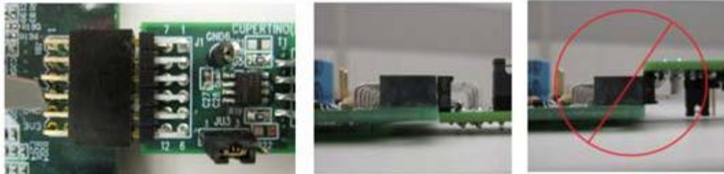
Figure 2. Pmod™ Connector Alignment
