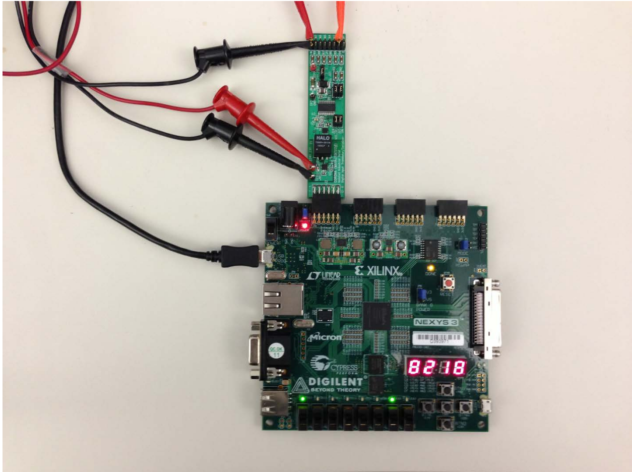
Figure 1. Corona Board Connected to Nexys 3 Development Kit
