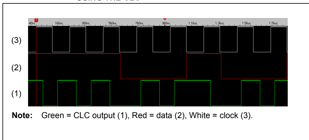
FIGURE 2-3: MANCHESTER LINE ENCODING FROM AN NRZ SOURCE USING THE CLC
