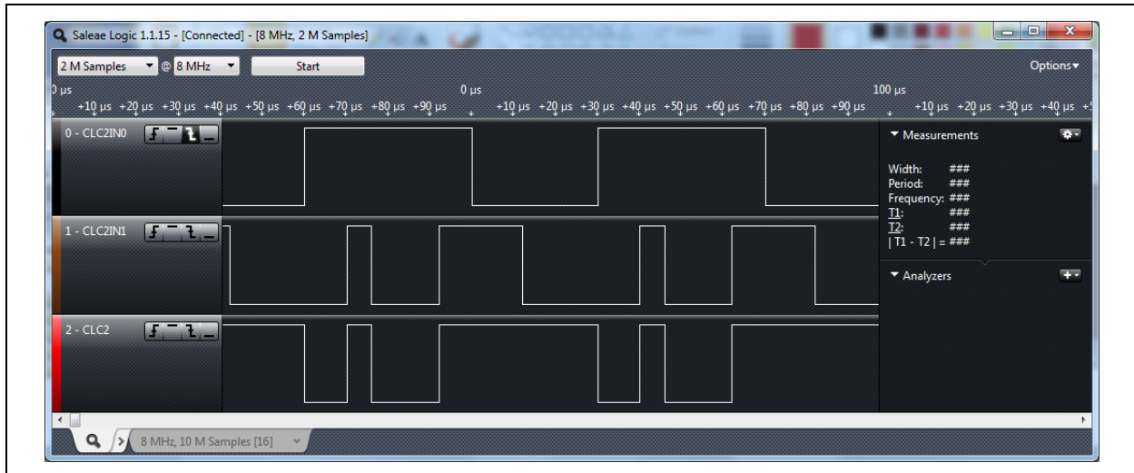
FIGURE B-17: D LTCH INPUT AND OUTPUT WAVEFORM EXAMPLE
