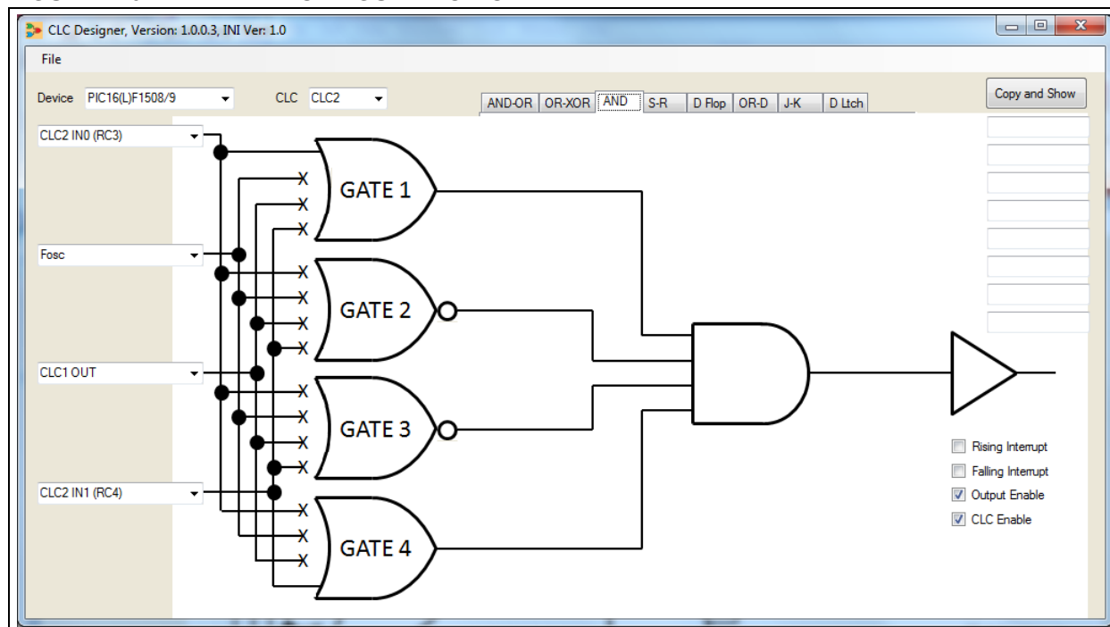
FIGURE B-6: AND CONFIGURATION OF CLC2
