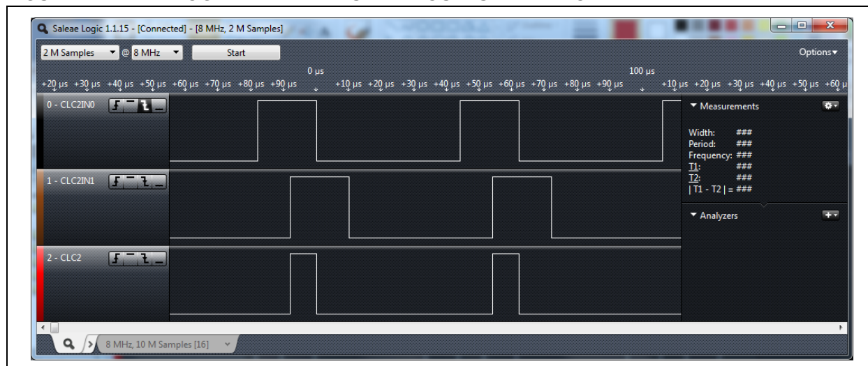
FIGURE B-7: LOGICAL 'AND' INPUT AND OUTPUT WAVEFORM EXAMPLE
