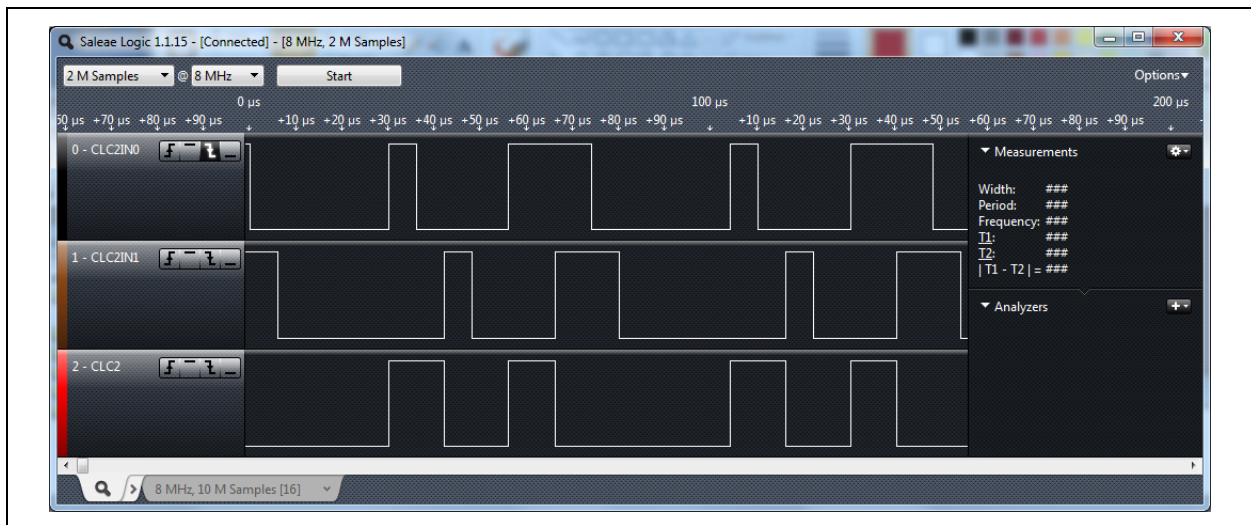
FIGURE B-9: S-R LATCH INPUT AND OUTPUT WAVEFORM EXAMPLE
