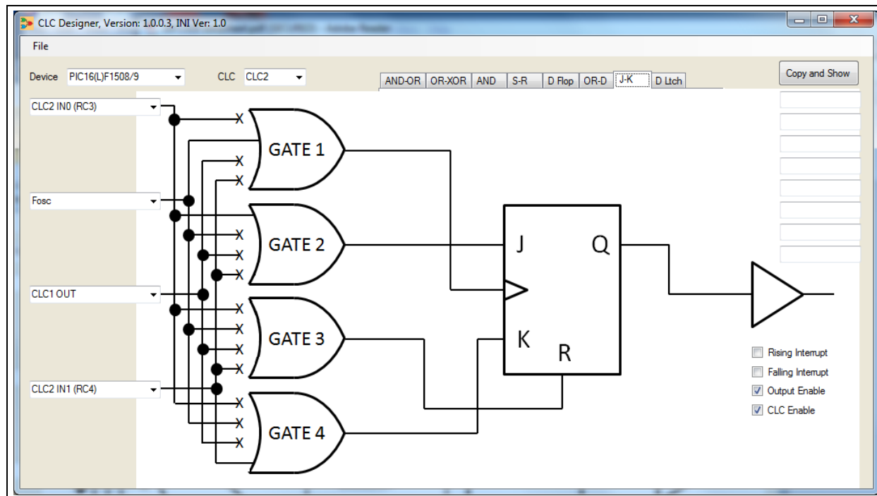
FIGURE B-14: J-K CONFIGURATION OF CLC2
