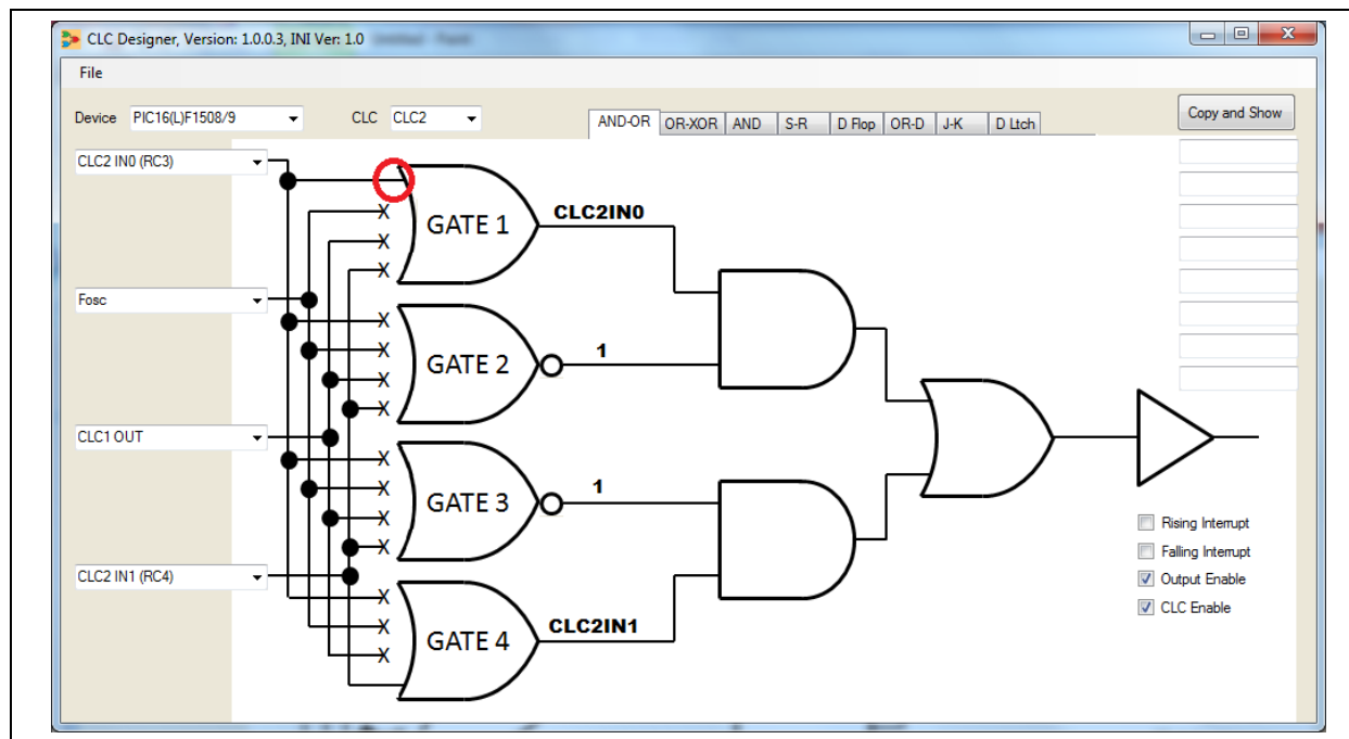
FIGURE B-2: AND-OR CONFIGURATION OF CLC2
