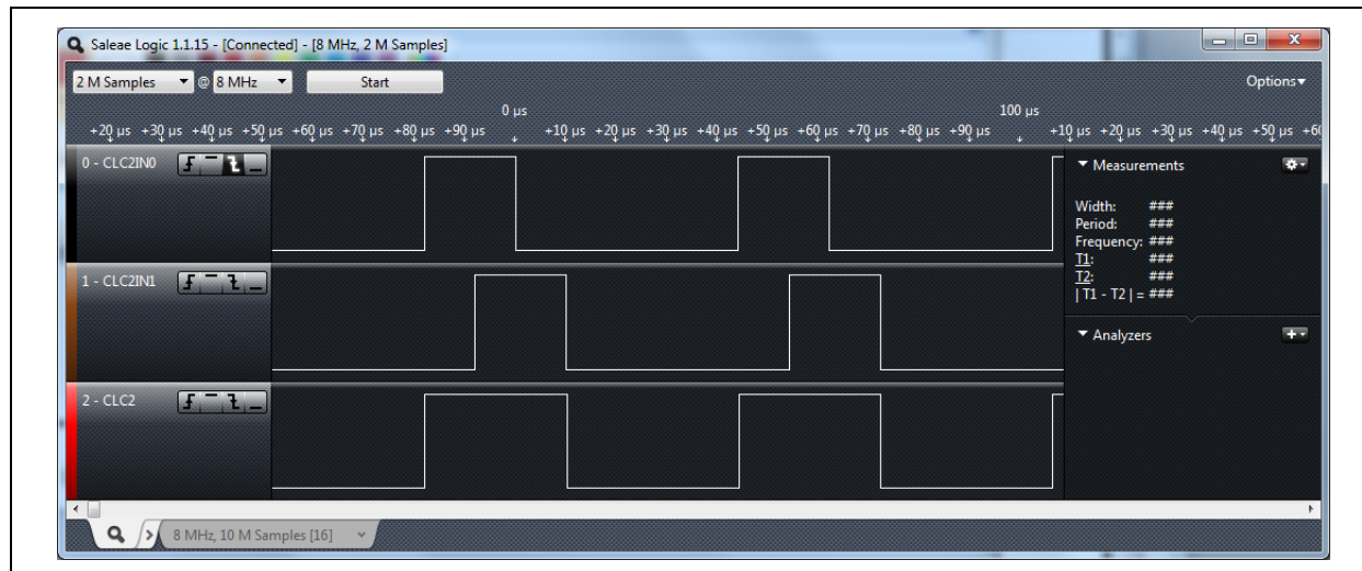
FIGURE B-3: LOGICAL 'OR' INPUT AND OUTPUT WAVEFORM EXAMPLE
