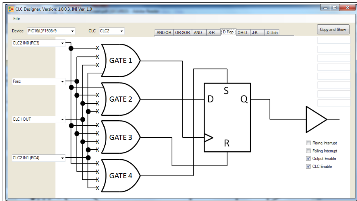
FIGURE B-10: D FLOP CONFIGURATION OF CLC2
