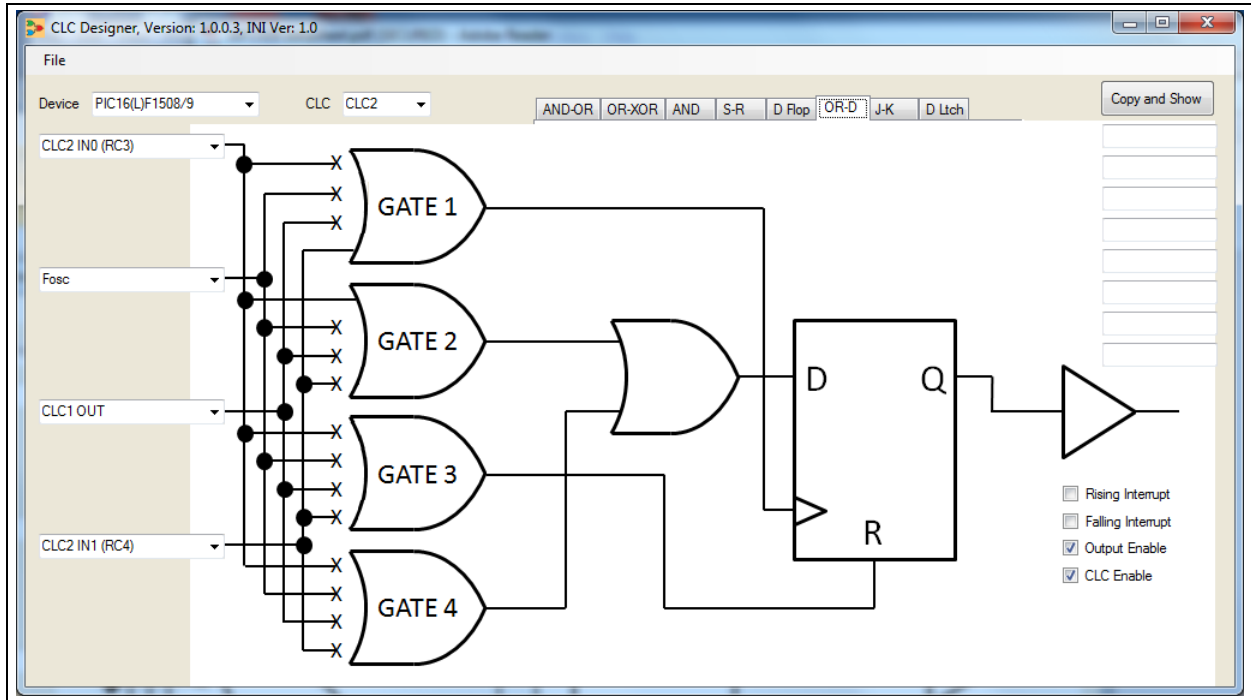
FIGURE B-12: OR-D CONFIGURATION OF CLC2
