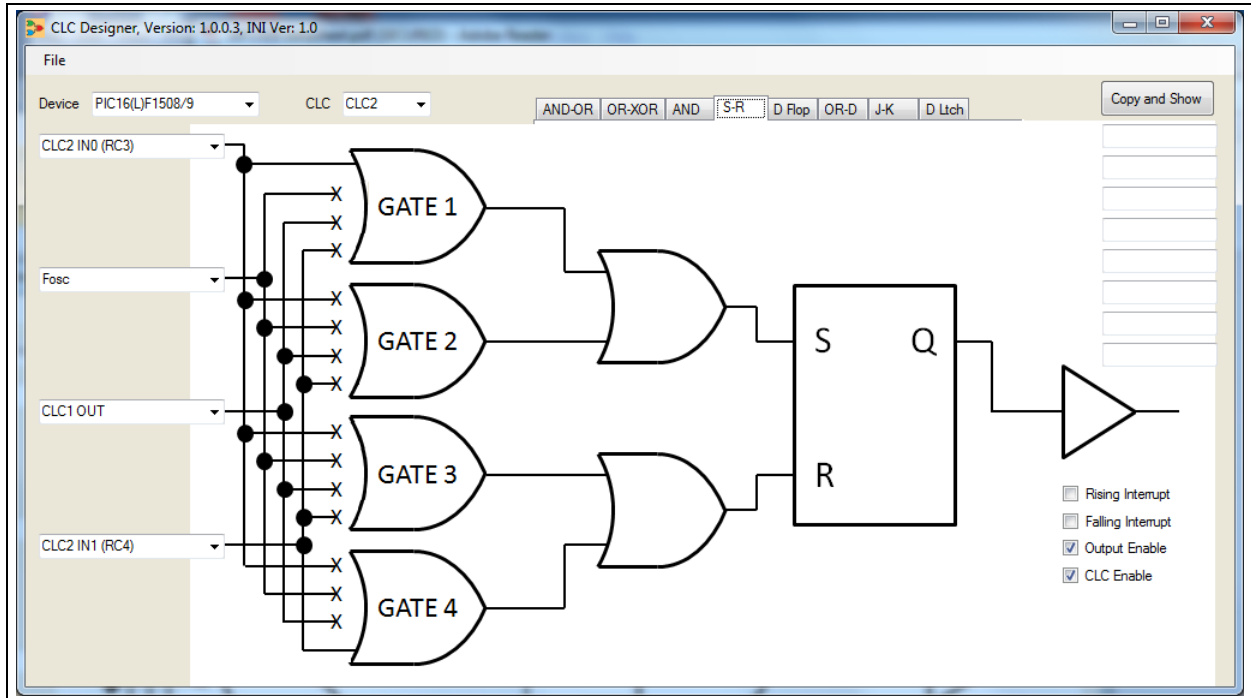
FIGURE B-8: S-R CONFIGURATION OF CLC2
