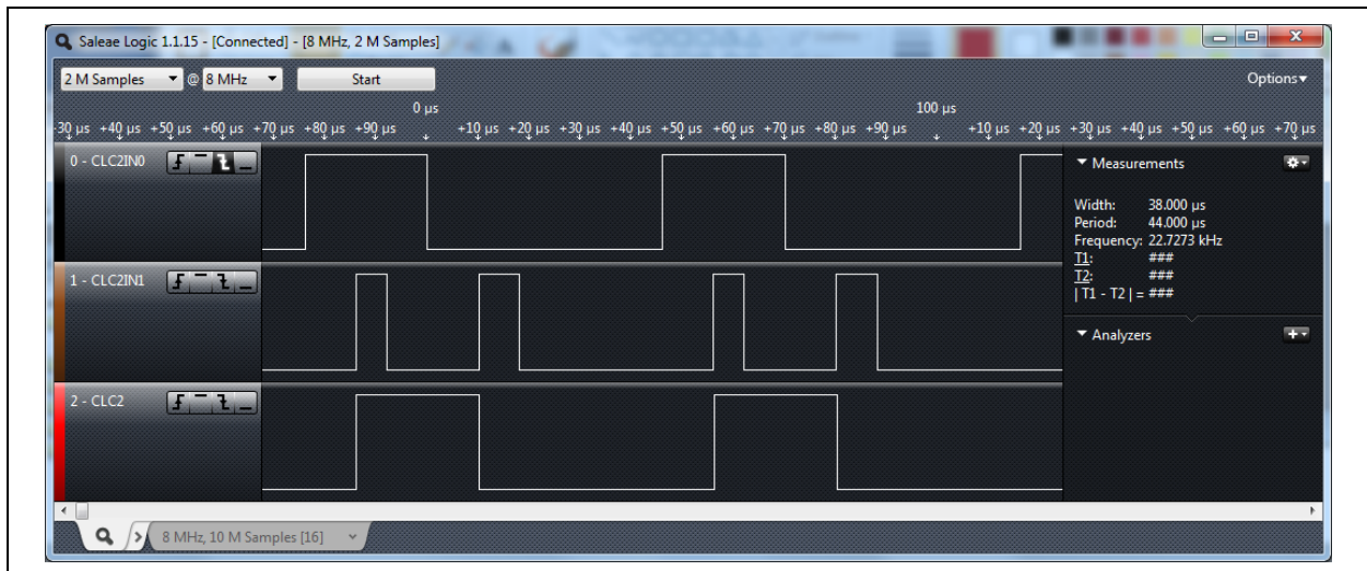
FIGURE B-13: OR-D INPUT AND OUTPUT WAVEFORM EXAMPLE
