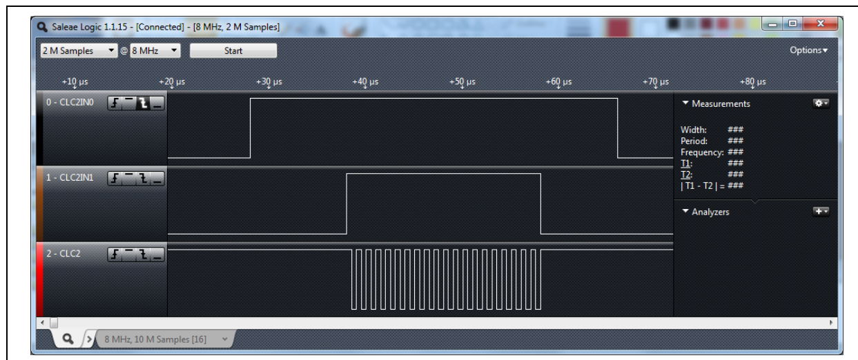
FIGURE B-15: J-K INPUT AND OUTPUT WAVEFORM EXAMPLE
