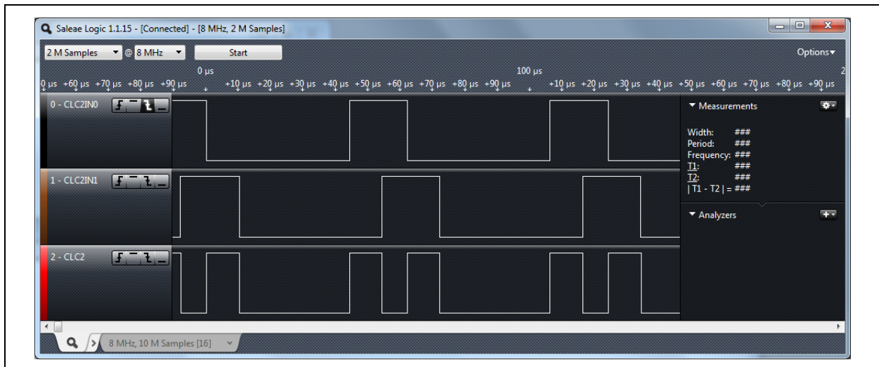
FIGURE B-5: LOGICAL 'XOR' INPUT AND OUTPUT WAVEFORM EXAMPLE
