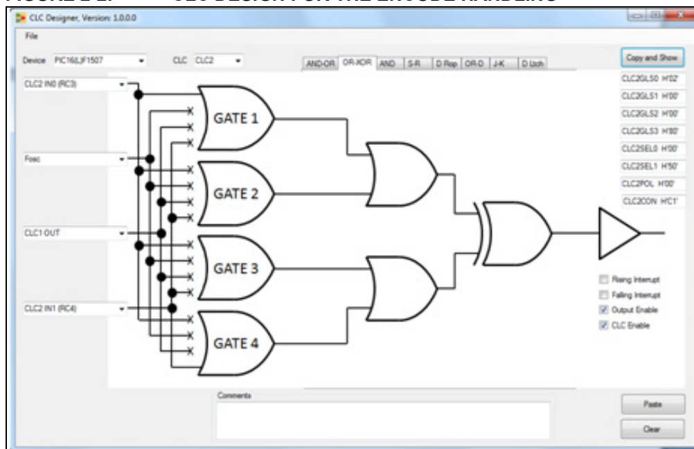
FIGURE 2-2: CLC DESIGN FOR THE ENCODE HANDLING
