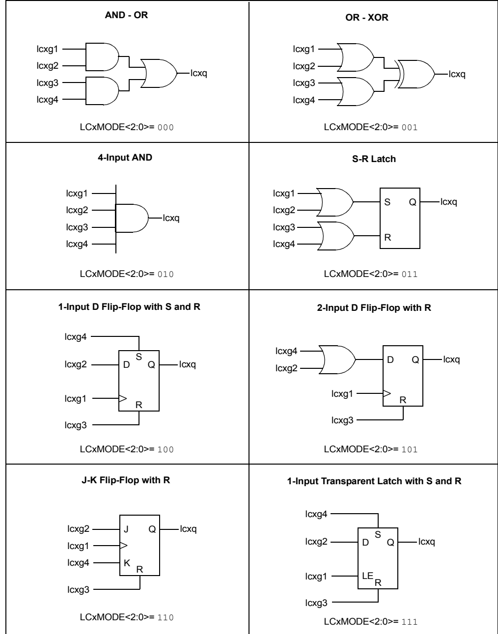
FIGURE 1-6: GATE INPUT/OUTPUT WITH INVERSION
