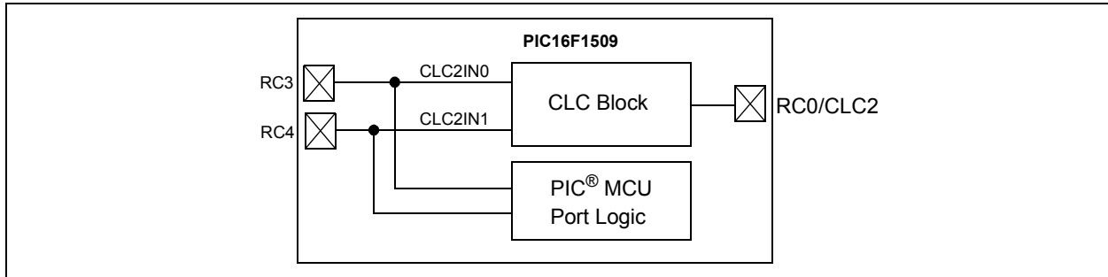
FIGURE B-1: BLOCK DIAGRAM SHOWING PORT SIGNALS FEEDING CLC BLOCK
