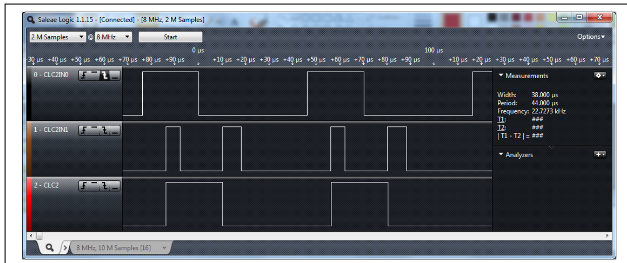
FIGURE B-11: D FLOP INPUT AND OUTPUT WAVEFORM EXAMPLE
