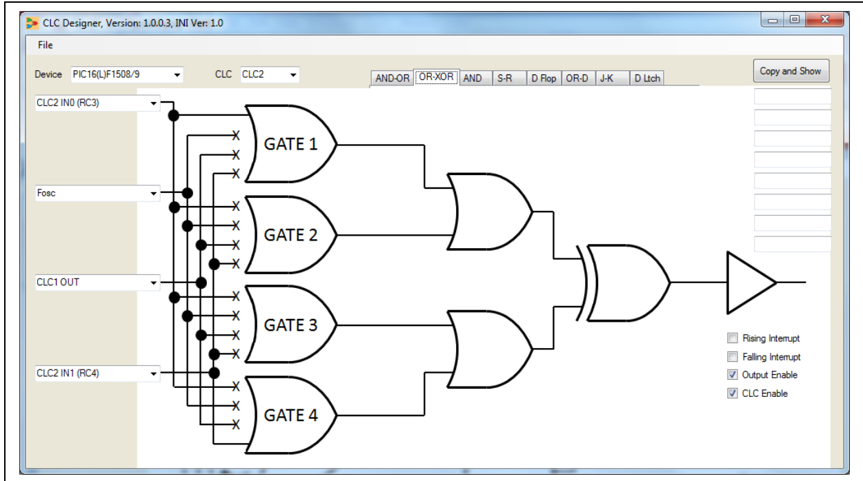
FIGURE B-4: OR-XOR CONFIGURATION OF CLC2
