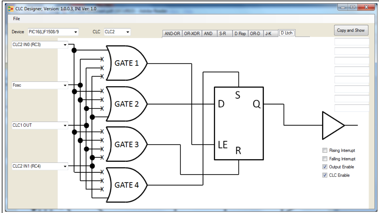
FIGURE B-16: D LTCH CONFIGURATION OF CLC2
