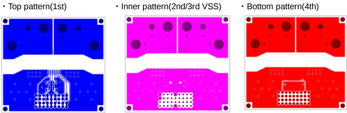
Figure 7. Board layout for measuring thermal resistance of CZ-3700
