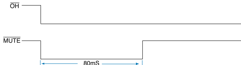
\overline{\text{MUTE}} and \overline{\text{OH}} Timing Figure 1
