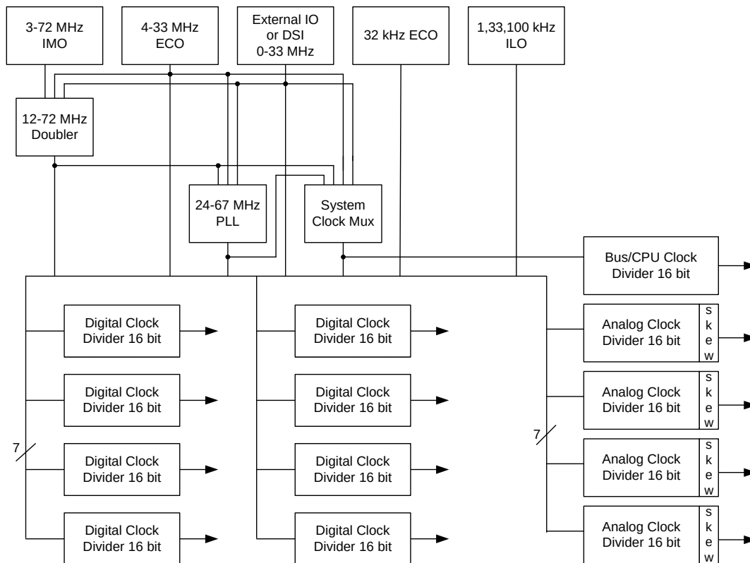
Figure 6-1. Clocking Subsystem
