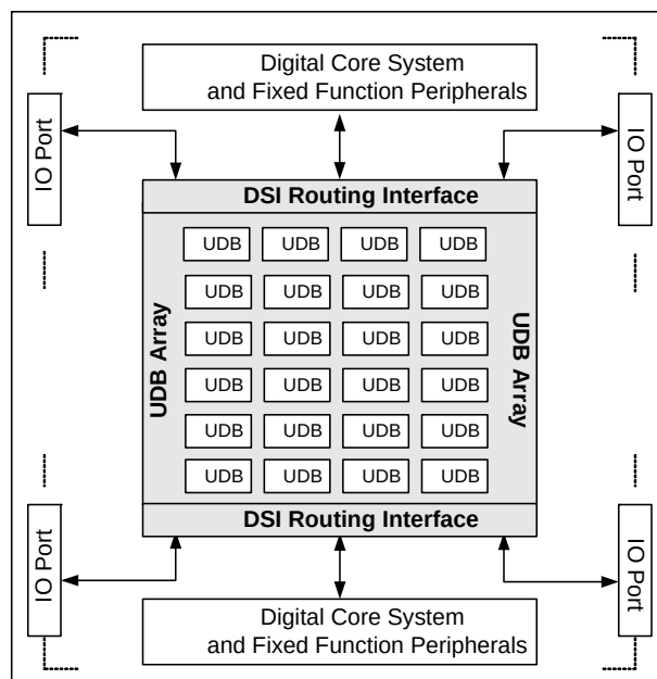
Figure 7-1. CY8C54 Digital Programmable Architecture
