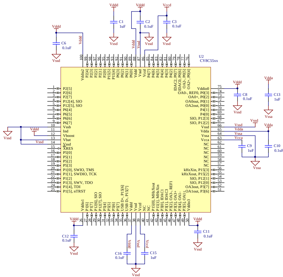
Figure 2-4. Example Schematic for 100-Pin TQFP Part with Power Connections
