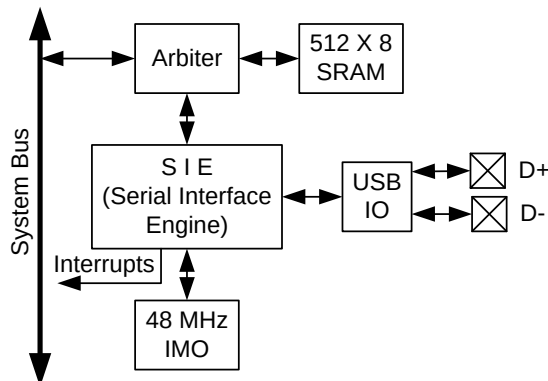
Figure 7-20. USB
