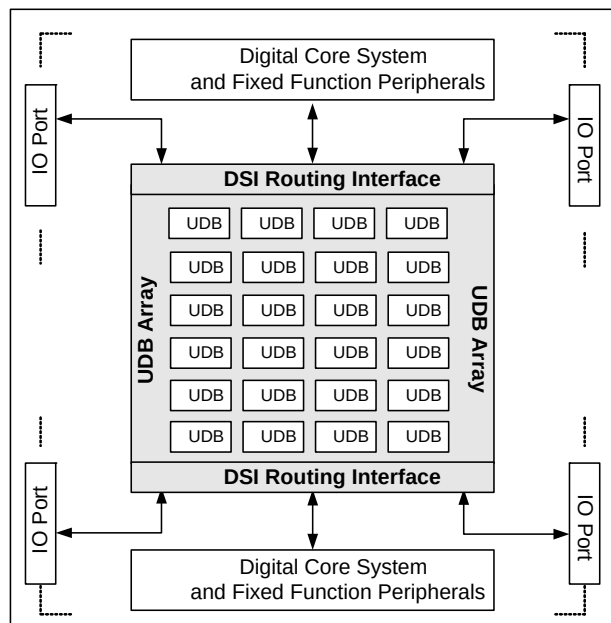
Figure 7-1. CY8C36 Digital Programmable Architecture
