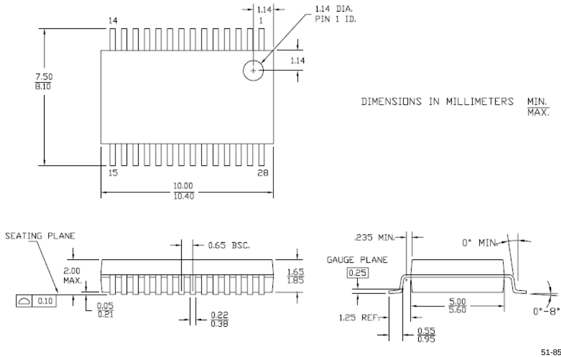
Figure 13. 28-Pin (210-Mil) SSOP
