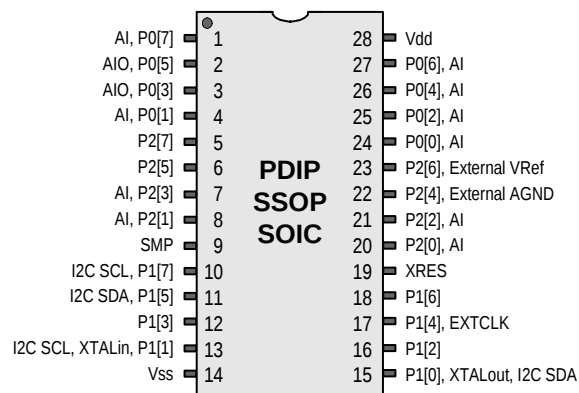
CY8C24423A 28-Pin PSoC Device
