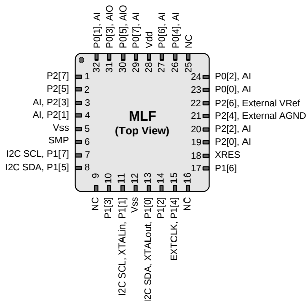
CY8C24423A 32-Pin PSoC Device
