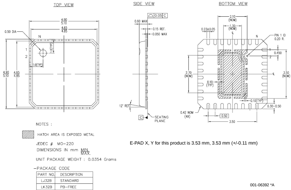
Figure 24. 32-Pin (5x5 mm 0.60 MAX) QFN
