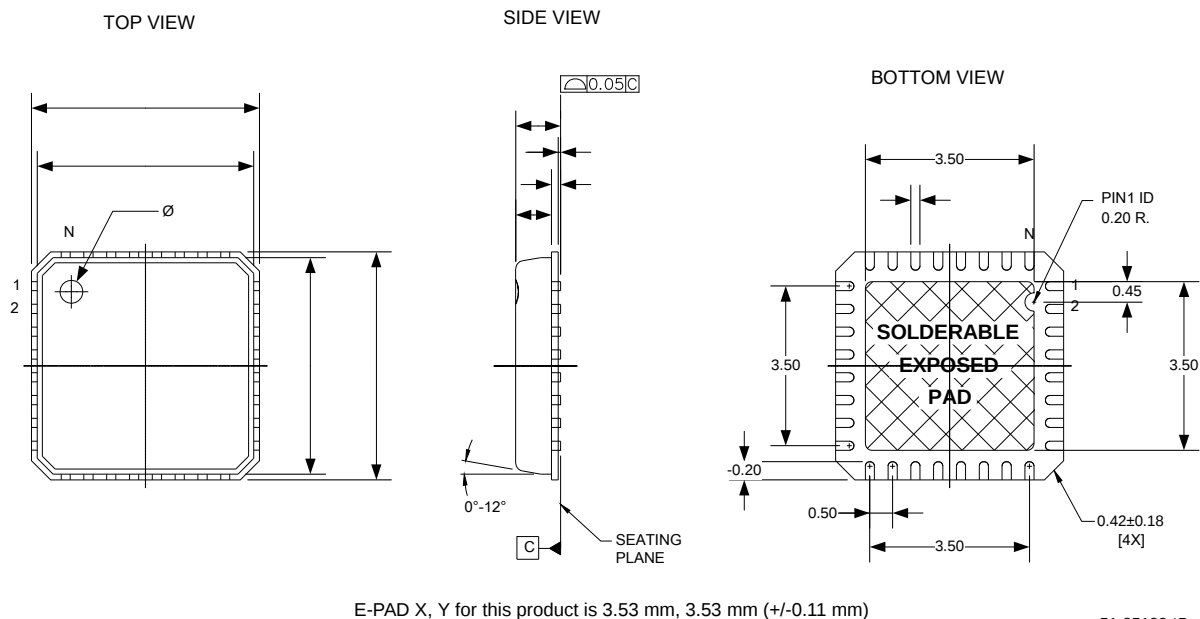
Figure 23. 32-Pin (5x5 mm 0.93 MAX) QFN
