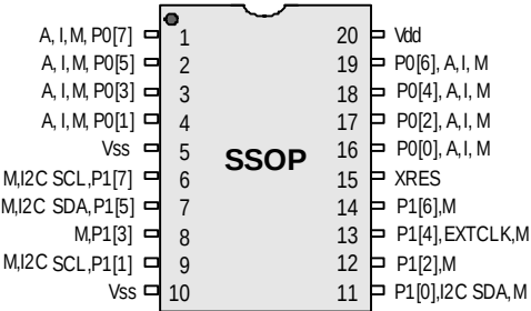
CY8C21334 20-Pin PSoC Device
