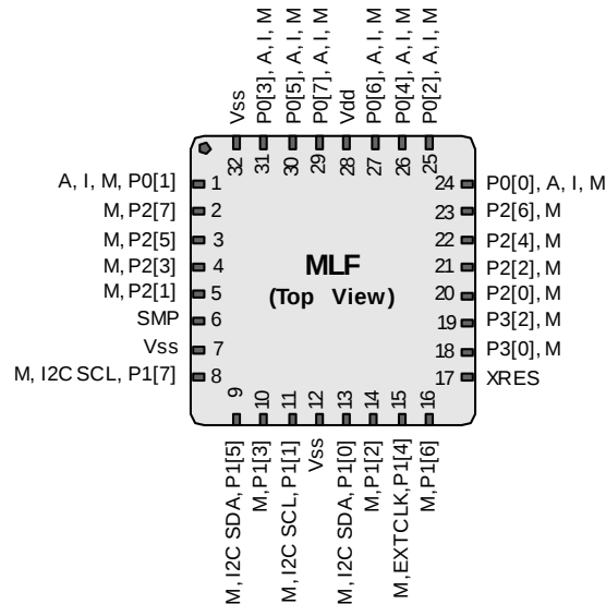
CY8C21634 32-Pin PSoc Device
