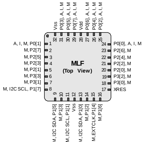
CY8C21434 32-Pin PSoc Device
