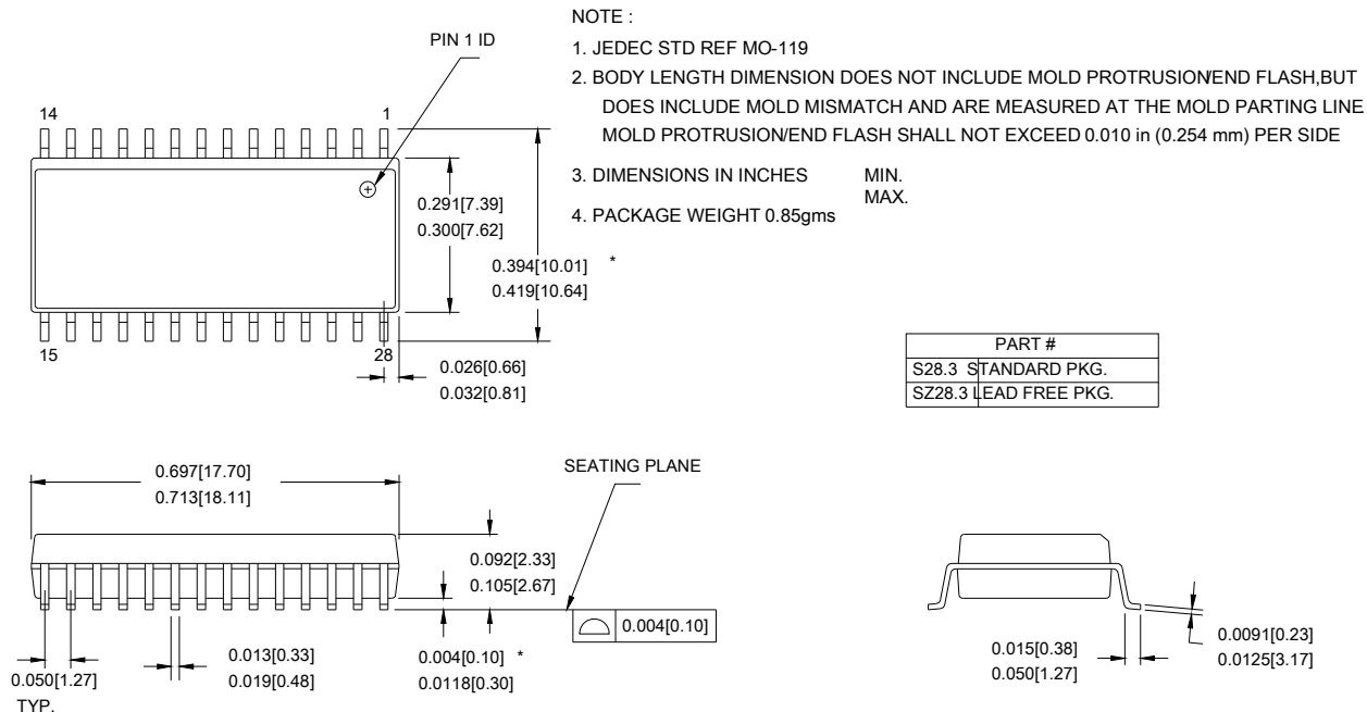
Figure 8. 28-Pin SOIC
