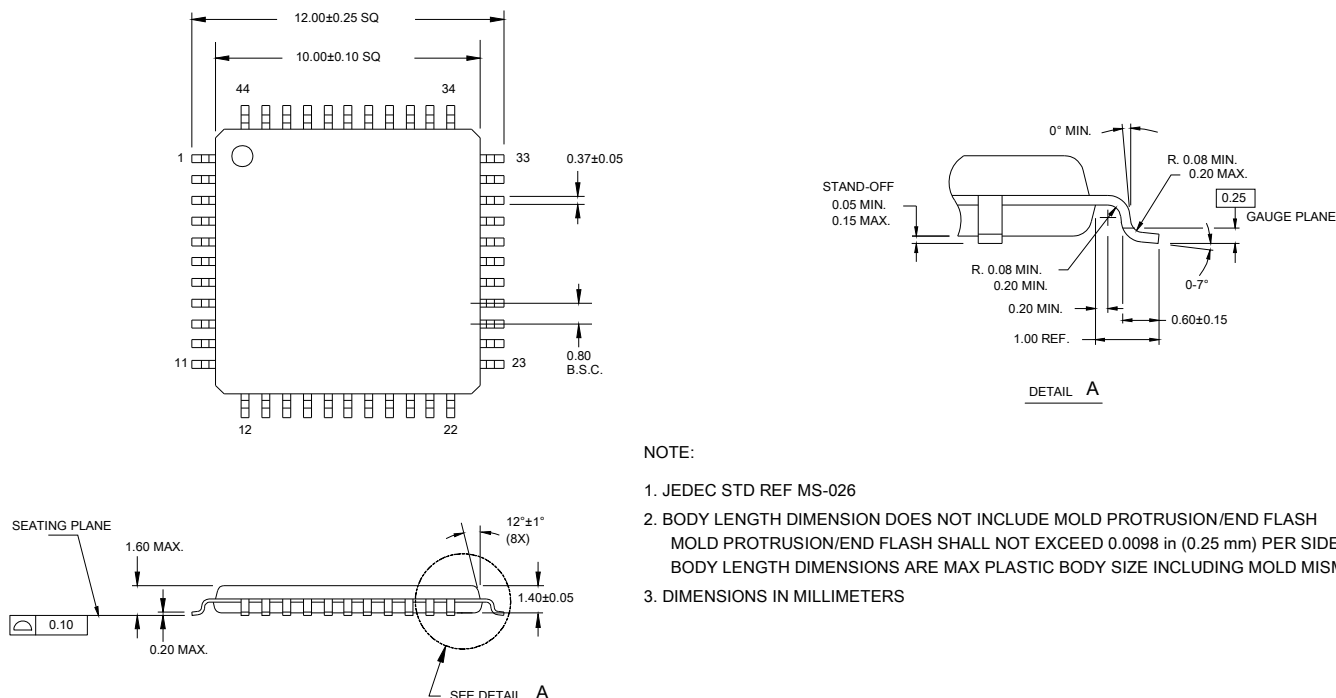
Figure 9. 44-Pin TQFP
