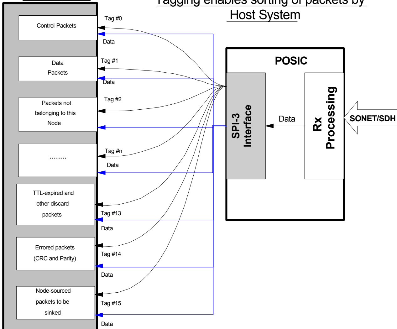
Figure 4. Frame Tagging Engine Data Sorting Diagram
