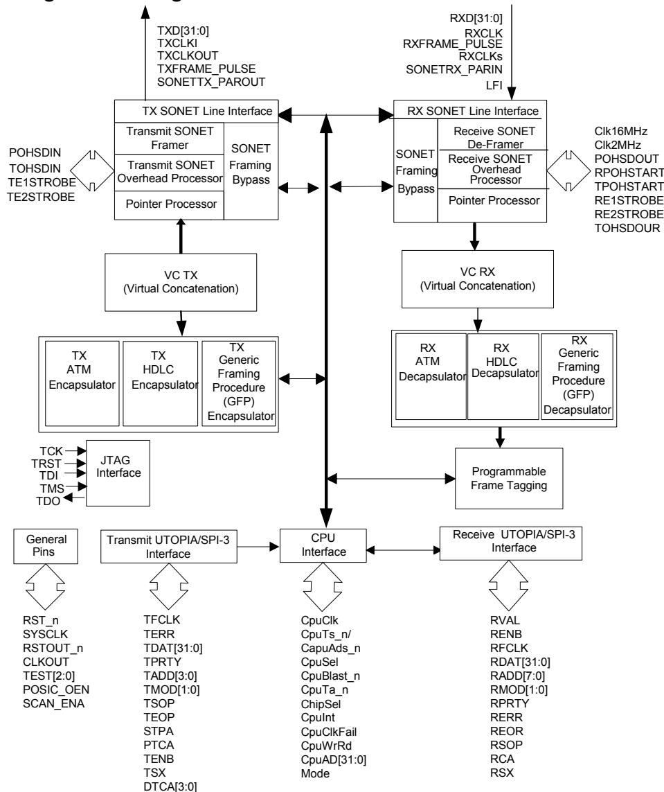
Figure 1. POSIC2GVC System Application Diagram
