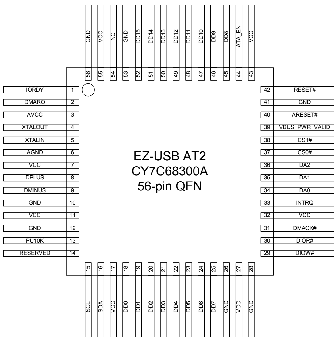
Figure 3-2. 56-pin QFN
