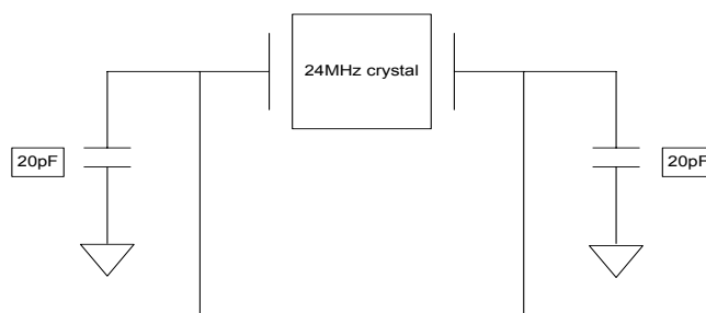
Figure 3-3. XTALIN, XTALOUT Diagram
