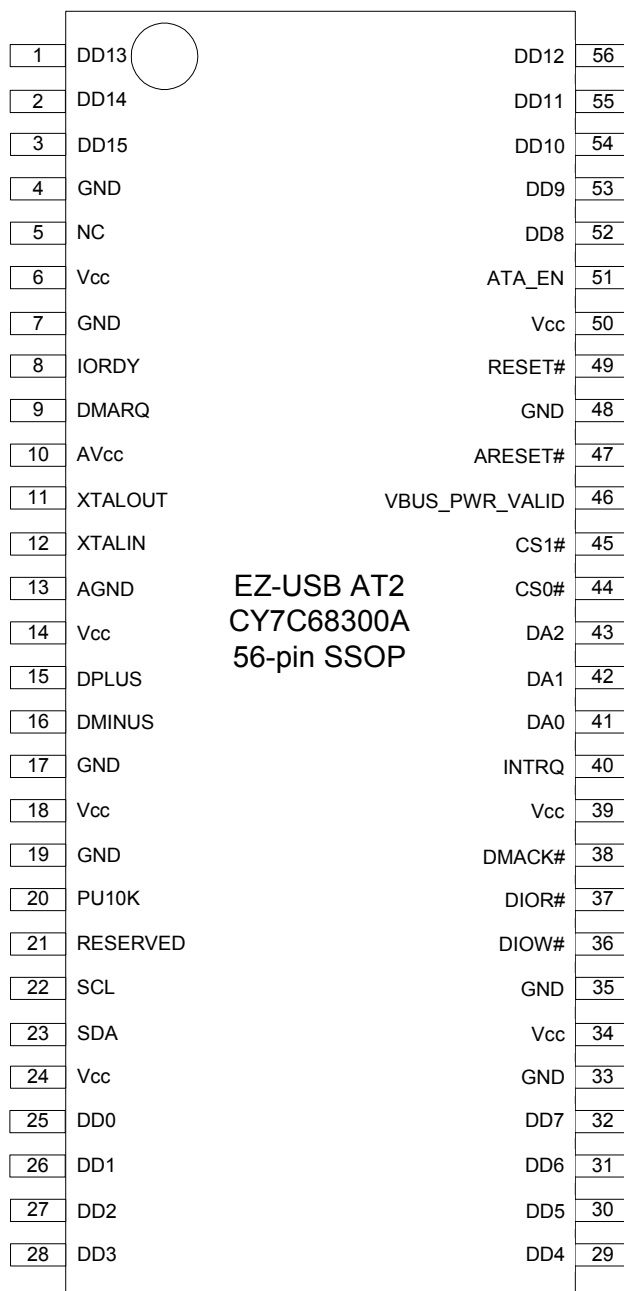
Figure 3-1. 56-pin SSOP
