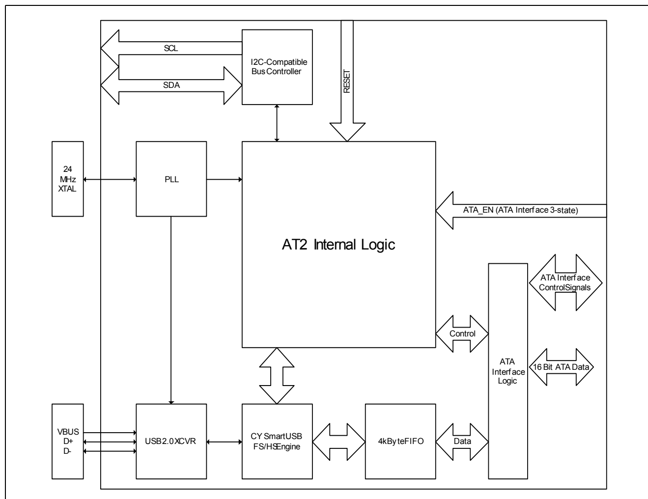
Figure 1-1. Block Diagram
