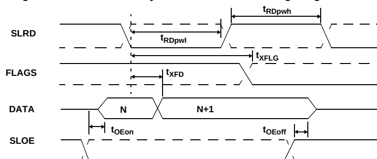
Figure 11. Slave FIFO Asynchronous Read Timing Diagram [13]
