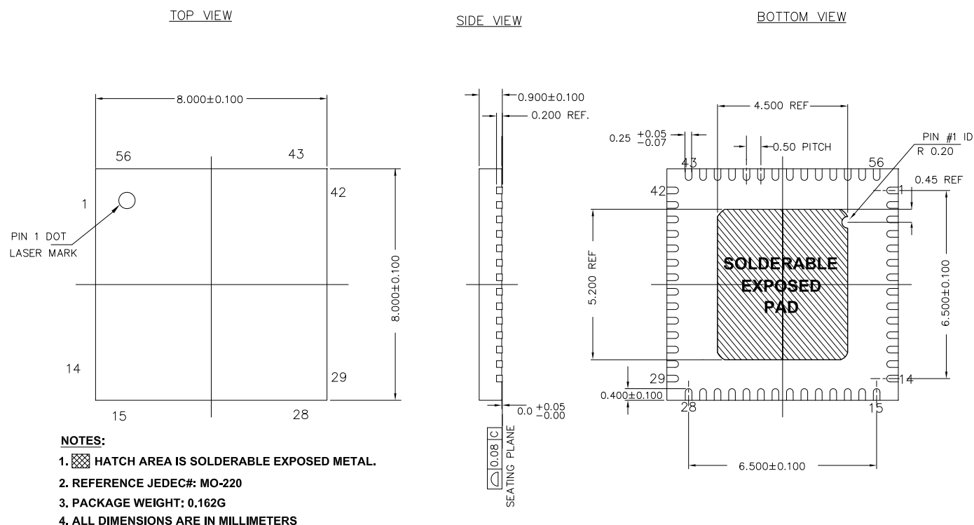
Figure 11-2. 56-Pin QFN 8 × 8 mm Sawn Version (001-53450)
