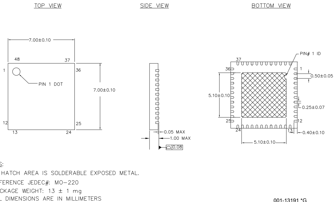
Figure 20. 48-pin QFN (7 × 7 × 1.00 mm) LT48A 5.1 × 5.1 E-Pad (Sawn) Package Outline, 001-13191
