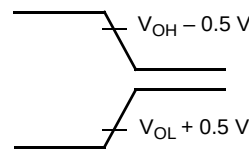
Figure 5. Test Point Levels for Driven-to-Three-State Time Measurements
