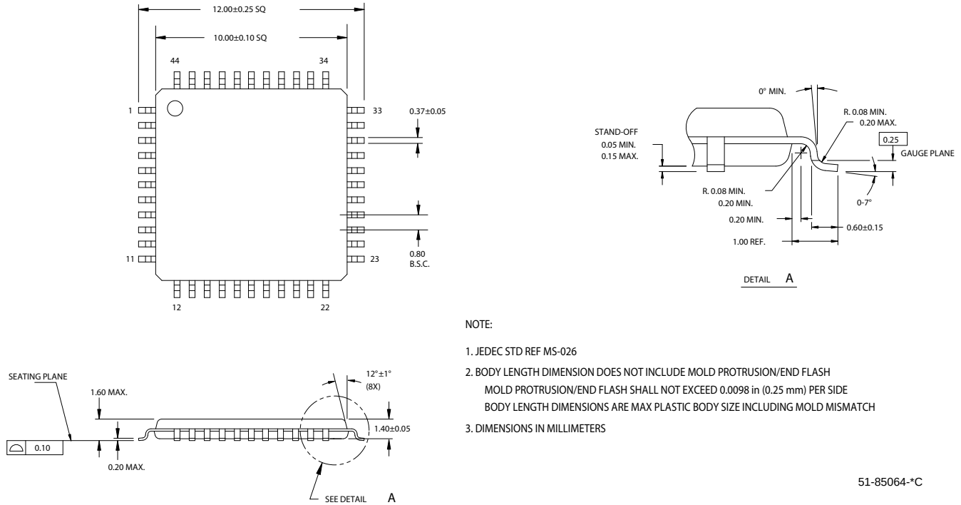
Figure 9. 44-Lead Thin Plastic Quad Flat Pack A44
