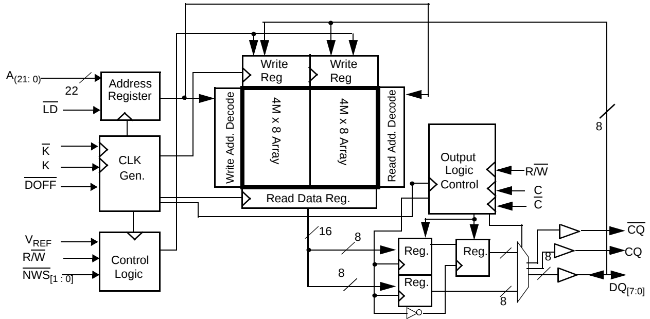
Logic Block Diagram (CY7C1516AV18)
