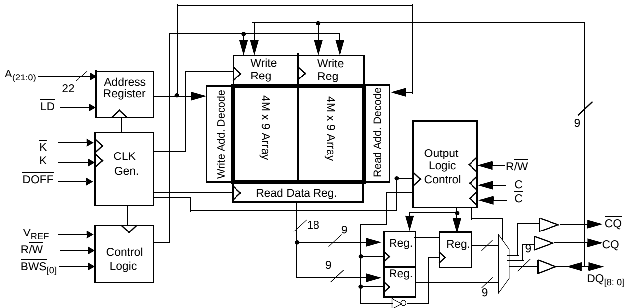
Logic Block Diagram (CY7C1527AV18)
