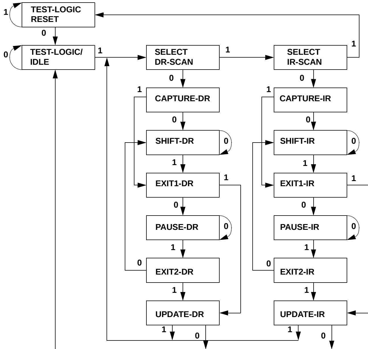
TAP Controller State Diagram [10]
