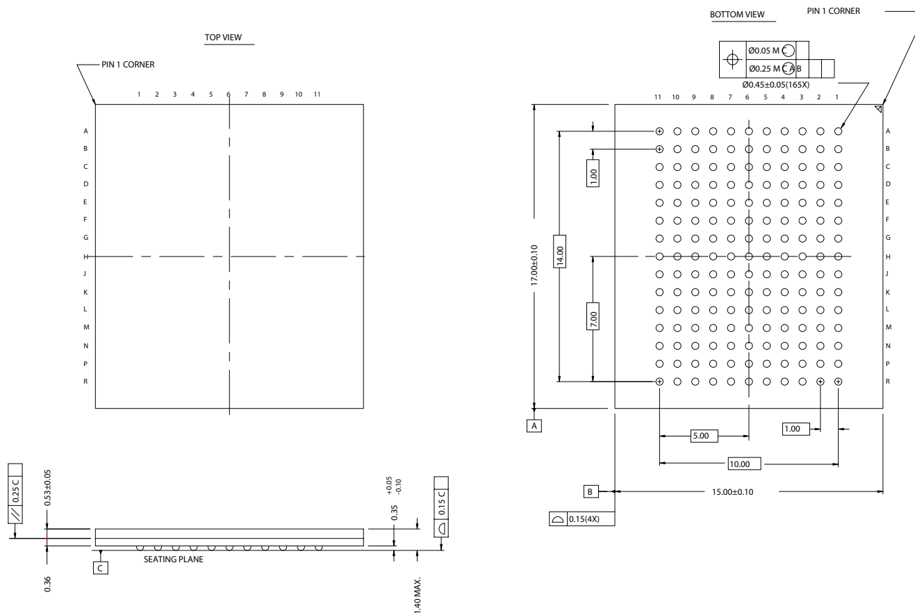
165-Ball FBGA (15 x 17 x 1.40 mm) BB165C
