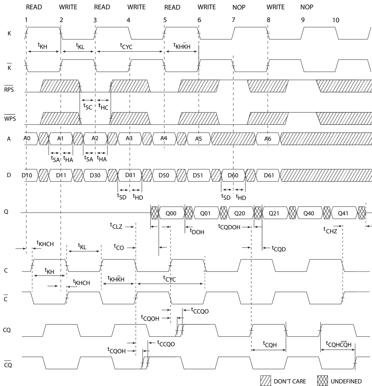
Figure 6. Read/Write/Deselect Sequence [36, 37, 38]
