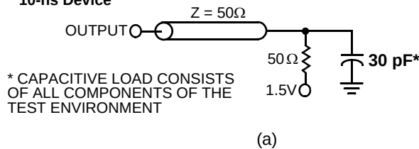
10-ns Device
