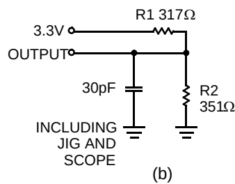
12-ns Device
