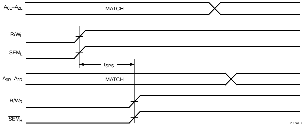
Timing Diagram of Read with \overline{\text{BUSY}} (M/ \overline{\text{S}} =HIGH) [20]
