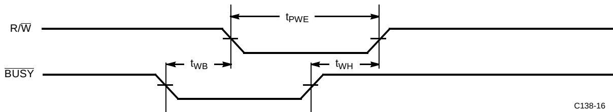
Write Timing with Busy Input (M/ \overline{\text{S}} =LOW)
