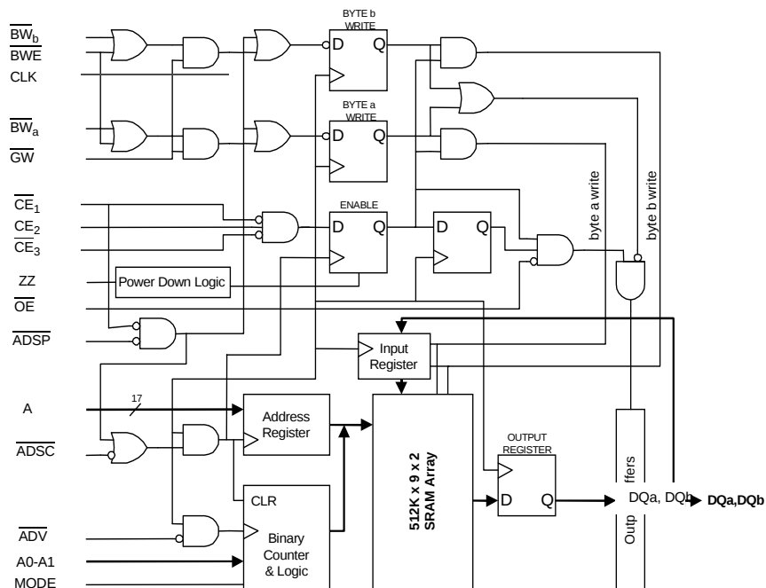
Functional Block Diagram—512K × 18 [1]
