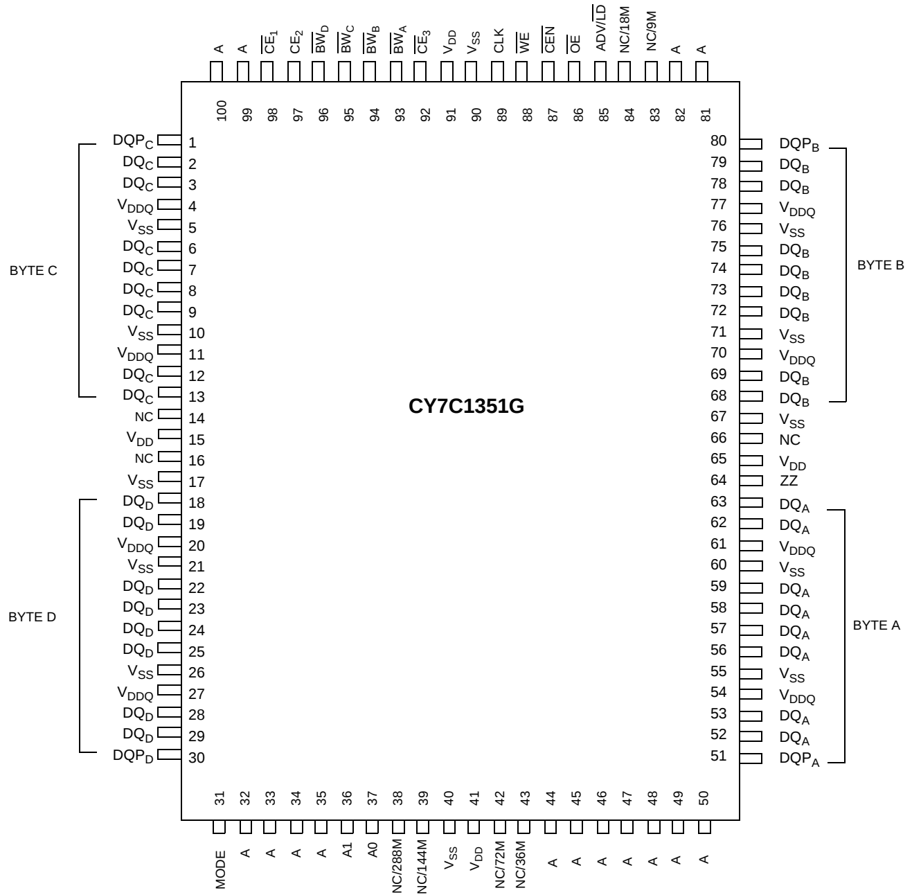
100-Pin TQFP Pinout
