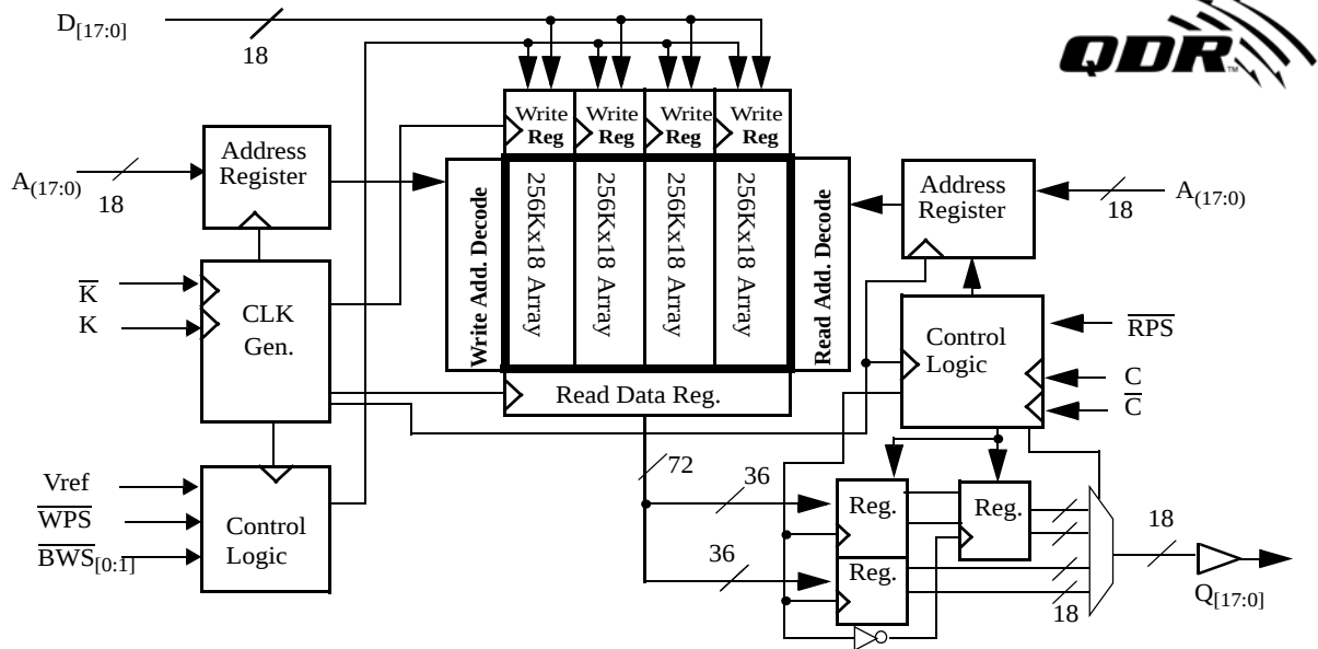
Logic Block Diagram (CY7C1307BV18)
