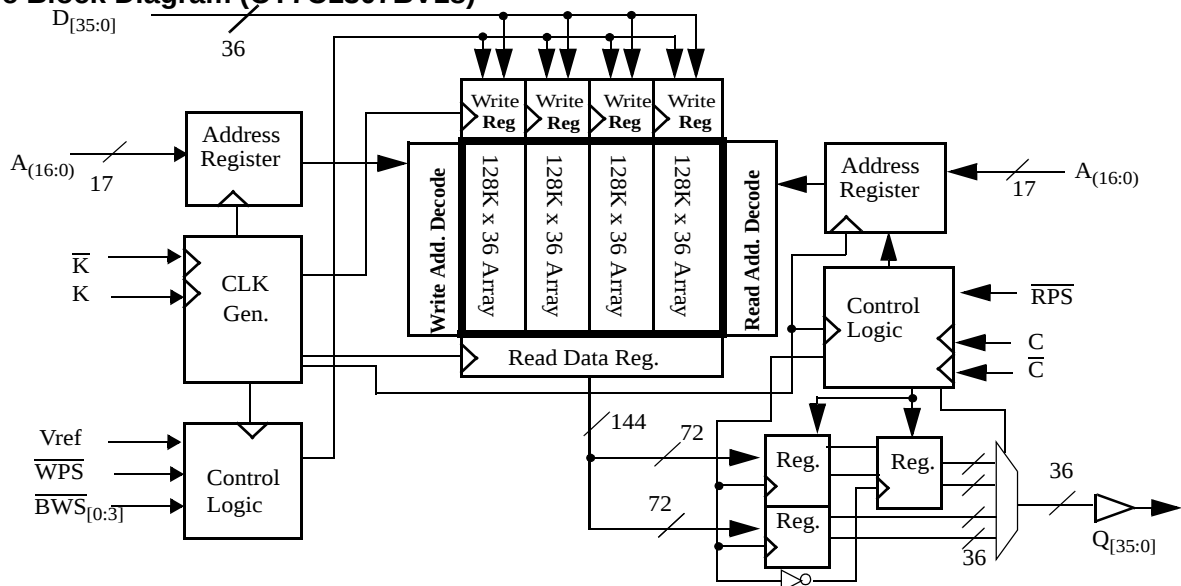
Logic Block Diagram (CY7C1307BV18)
