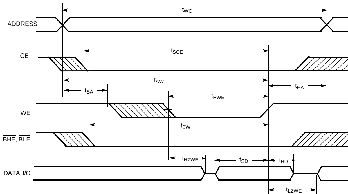
Write Cycle No. 3 ( \overline{\text{WE}} Controlled) \overline{\text{OE}} LOW)
