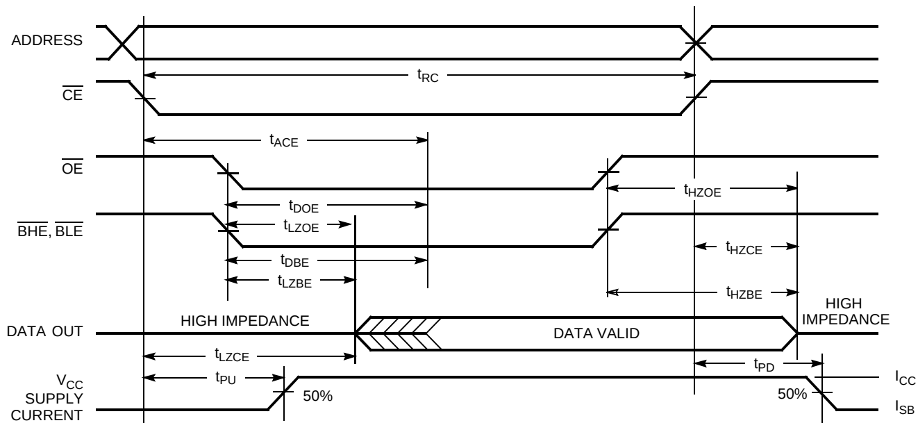
Figure 6. Read Cycle No. 2 ( \overline{\text{OE}} Controlled) [11, 12]
