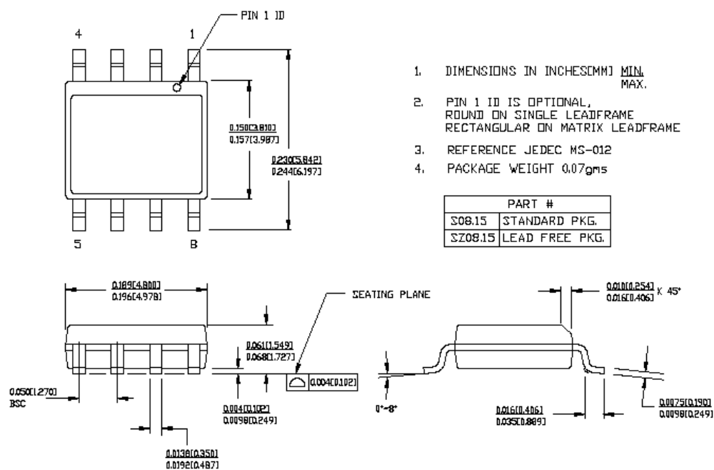
Figure 8. 8-pin (150-Mil) SOIC S8
