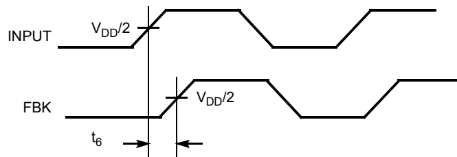
Figure 5. Input to Output Propagation Delay
