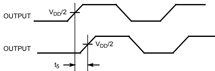
Figure 4. Output to Output Skew
