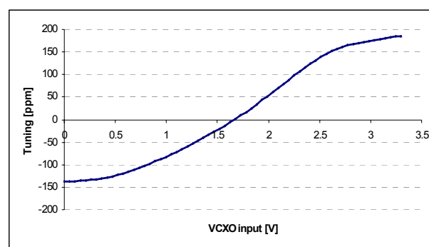
Figure 1. VCXO Profile
