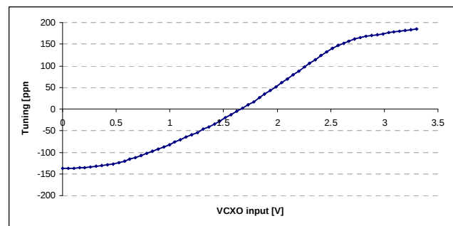
Figure 2. VCXO Profile
