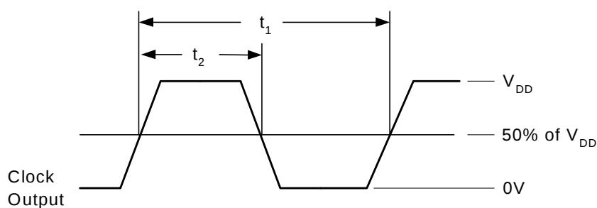
Figure 4. Duty Cycle Definition
