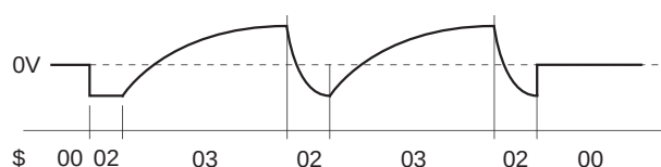
Fig. 2. Constructing the search voltage by alternating between $02 and $03. (Voltage at Pin 5)
