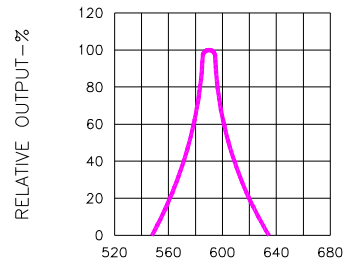
Fig.2 SPECTRAL RESPONSE
