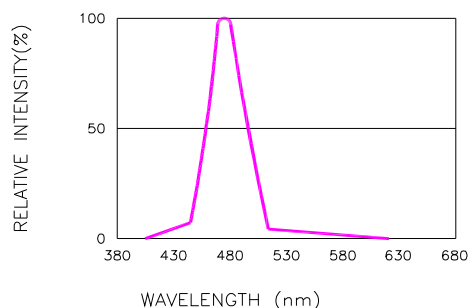
Fig.2 RELATIVE INTENSITY VS. WAVELENGTH
