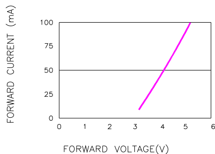
Fig.6 PEAK FORWARD VOLTAGE VS. FORWARD (100us TEST PULSE, 1% DUTY CYCLE)
