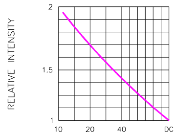
Fig.5 LUMINOUS INTENSITY VS. DUTY CYCLE (AVERAGE If=10mA)
