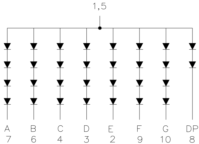
CSS-2318 Common Anode (CSS-2319 Common Cathode.)
