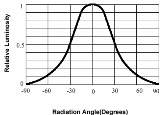
Fig 6. Relative Power vs. Radiation Angle
