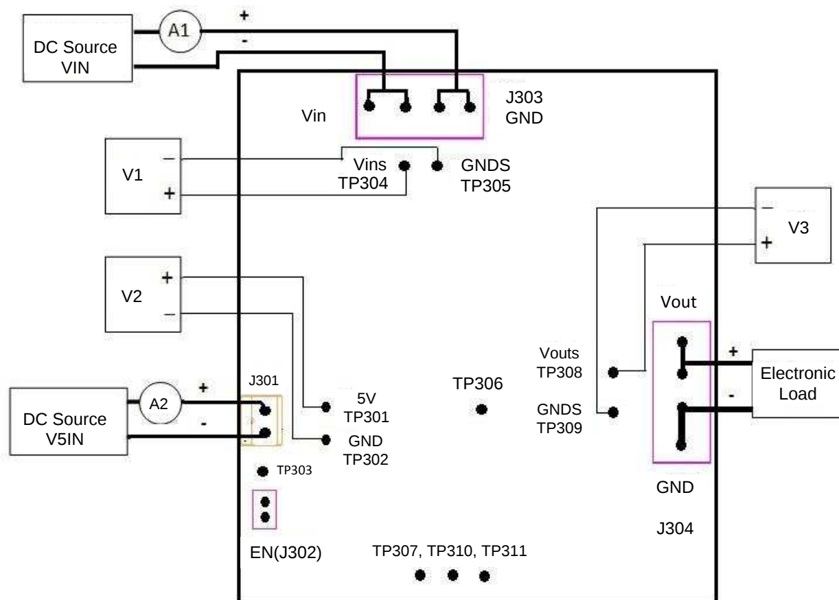
Figure 3. CSD87588NEVM-603 Recommended Test Setup
