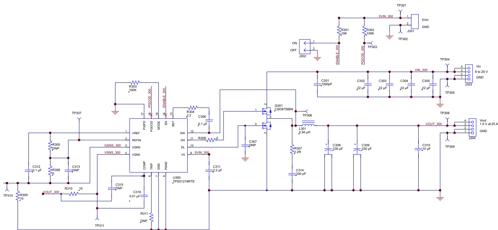
Figure 1. CSD87588NEVM-603 Schematic
