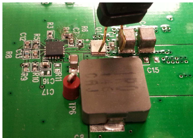
Figure 2. Tip and Barrel Measurement for Vsw Waveform
