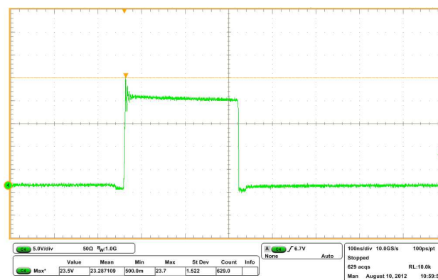
Figure 6. Switching Node Waveform, VIN = 19 V, Iout = 10 A
